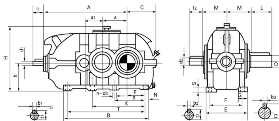
外形及安装尺寸 Appearance and installation dimensions
