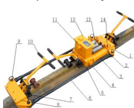
YTF-400 Ⅱ 型液压轨缝调整器 Hydraulic Rail Gap Adjuster
