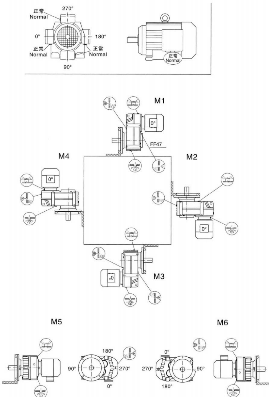
FF/FAF/FAZ37-157安装形式图 FF/FAF/FAZ Mounting position example
