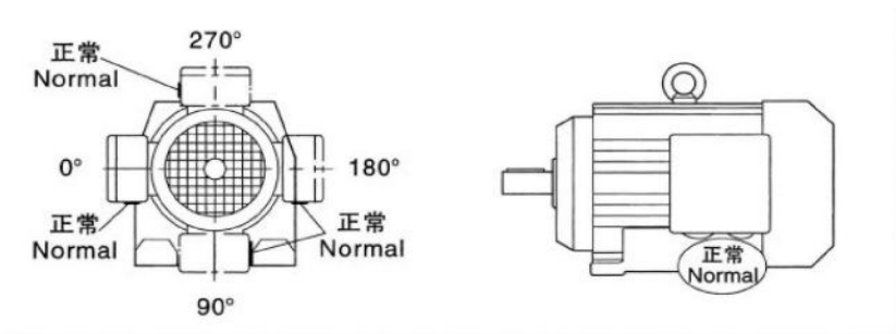
KAT37-157安装形式图 KAT37-157 Mounting position example
