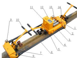
YTF-400 Ⅱ 型液压轨缝调整器 Hydraulic Rail Gap Adjuster
