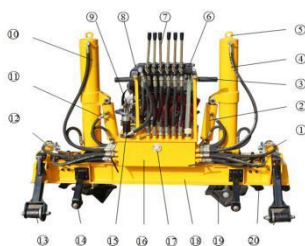
YQBJ-300x200 型液压起拨道机 Hydraulic Track Lifting Machine
