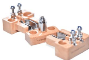
动静插头组 Dynamic And Static Plug Assembly
